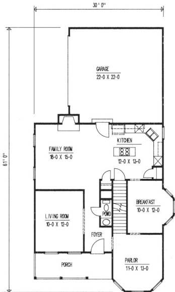
FIRST FLOOR PLAN (WITH OPTIONAL GARAGE)
