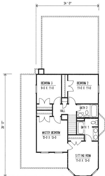
SECOND FLOOR PLAN (WITH OPTIONAL GARAGE)
