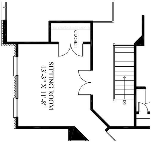
PARTIAL SECOND FLOOR PLAN W/ OPT. SITTING ROOM PLAN
